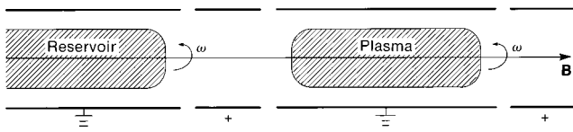
FIG. 20. Plasma in thermal contact with heat and angular momentum reservoir.
