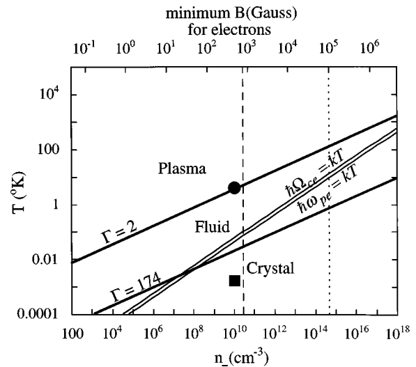
FIG. 21. Phase diagram of the one-component plasma: temperature T vs density n_- . Also shown on upper x axis is the minimum magnetic field required to produce the corresponding density, B = \sqrt{8\pi mn_- c^2} [see Eq. (3.21)].
