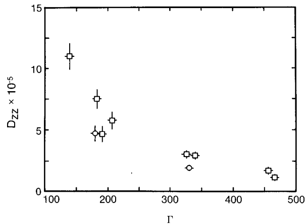
FIG. 28. Average single-particle diffusion in z direction as a function of \Gamma in spherical plasmas. Squares N=100 ; circles N=256 ; \Omega_c/\omega_z=10 . Position is measured in units of (3e^2/m\omega_z^2)^{1/3} , time is in units of \omega_z^{-1} . From Dubin and O'Neil (1988).
