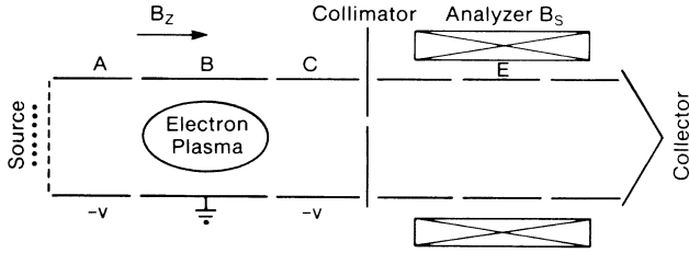
FIG. 1. The cylindrical containment apparatus.
