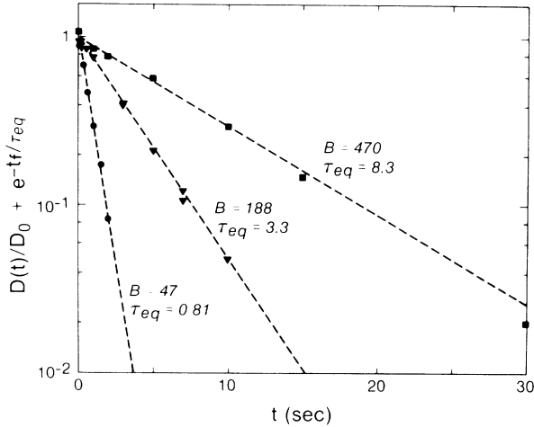
FIG. 3. Measured "distance" from equilibrium D(t) vs time for B=47, 188, and 470 G. The dashed lines show exponential fits to obtain \tau_{eq} .
