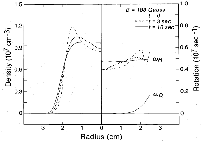
FIG. 2. Experimental plasma density profiles n(r,t) and rotation profiles \omega_R(r,t) at three different times t , showing the evolution to equilibrium. Also shown is the diamagnetic drift \omega_D(r) at t = 10 sec.
