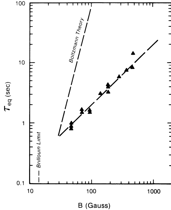
FIG. 4. Experimental density equilibration times \tau_{eq} vs magnetic field B . The dashed line through the data represents \tau_{eq} \propto B^1 ; the upper dashed line is the prediction of traditional Boltzmann theory, scaling as B^4 .
