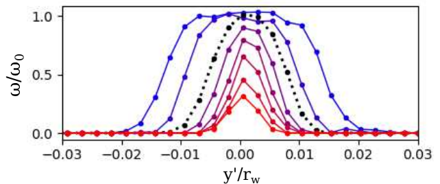
FIG. 4. Measurements of the filament profile \omega(x' = 0, y') for the initial vortex [cf. Fig. 2(a,b)] subjected to an external strain flow with \epsilon^* = 0.377 for time intervals \Delta t^* = 7.2 - 13.5 (blue to red). The initial filament used in the experiments ( \Delta t^* = 9 ) is shown as a dotted line, and circles indicate pixel locations.
