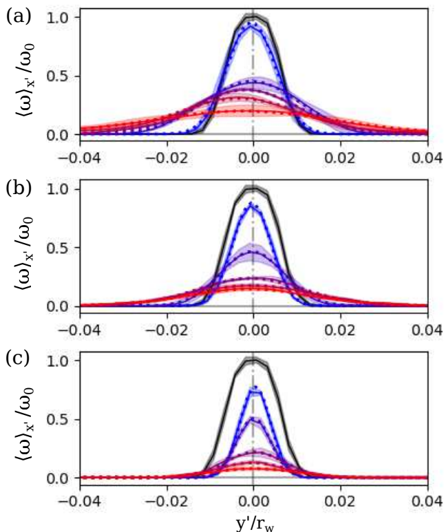
FIG. 16. The mean vorticity profile perpendicular to the filament (i.e., averaged over the x' direction), for \epsilon^* = (a) 0, (b) 0.015, and (c) 0.03, at times t^* = 0 (black), 22.5, 31.5, 40.5, 49.5, and 58.5 (blue to red). Solid lines and shaded regions indicate the average and standard deviation of five identical runs. Dotted lines indicate Gaussian fits to the data.
