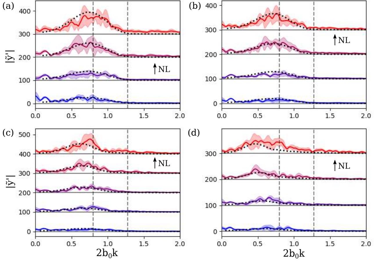
FIG. 10. Experimental wave spectra |\tilde{y}'| [cf. Eq. (20)] are compared to predictions of a contour dynamics model described by Eqs. (12) (dotted) for (a) \epsilon^* = 0 , t^* = 22.5, 24.75, 27, 29.25 ; (b) \epsilon^* = 0.01 , t^* = 22.5, 24.75, 27, 29.25 ; (c) \epsilon^* = 0.02 , t^* = 22.5, 24.75, 27, 29.25, 31.5 ; (d) \epsilon^* = 0.03 , t^* = 22.5, 27, 31.5, 36 . Time proceeds upwards in each panel from blue to red, separated for clarity by intervals of \Delta|\tilde{y}'| = 100 . The nonlinear transition [cf. Eq. (17)] is indicated (NL), as are k_m and k_c (dashed lines). Shaded regions indicate the experimental uncertainty.
