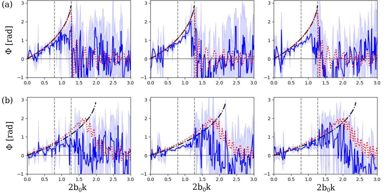
FIG. 11. Measured phase shift between the upper and lower filament boundaries as a function of wavenumber for (a) \epsilon^* = 0 , t^* = 22.5, 24.75, 27 ; (b) \epsilon^* = 0.02 , t^* = 22.5, 27, 31.5 . Also shown are predictions of Eq. (14) where k is scaled by \exp(\epsilon t) (black, dash-dot), and solutions to the linear contour dynamics model [Eq. (12)] averaged over initial phase (red, dotted). Shaded regions indicate the experimental uncertainty, k_m and k_c are indicated (dashed lines), and for \epsilon^* \neq 0 instability is predicted for k < k_c \exp(\epsilon t) .
