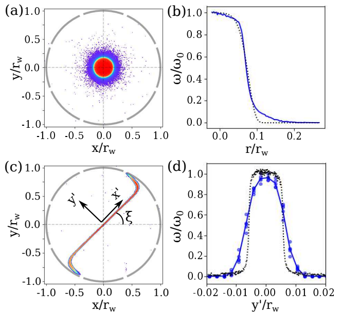
FIG. 2. Measurements of the initial vortex and filament used in the experiments. (a) CCD image of the initial axisymmetric vortex just prior to application of the strain flow, where data are truncated for \omega < 0.03\omega_0 ; (b) radial vorticity profile \omega(r) (blue) corresponding to panel (a), along with a fit to Eq. (6) (dotted); (c) CCD image of the initial filament following application of a strong external strain flow, with the filament angle \xi and filament-aligned coordinate system (x', y') indicated; and (d) cross-section of the filament as measured by the CCD (blue), and that obtained by scaling the profile in panel (b) according to Eq. (7) (black).
