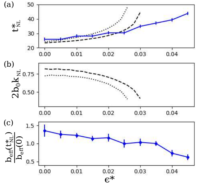
FIG. 15. Measurements (error bars) and predictions of the linear model (black lines) showing (a) the time t_{\text{NL}}^* at which nonlinearity becomes important [as defined by Eq. (17)] versus \epsilon^* ; (b) the wavenumber k_{\text{NL}} for which Eq. (17) is first satisfied in the model; and (c) the effective half-width b_{\text{eff}}(t_{\text{NL}}^*) at the onset of nonlinearity. The model is averaged over initial phase and plotted for s(0) = 0.01 (dotted) and s(0) = 0.03b_0k (dashed).
