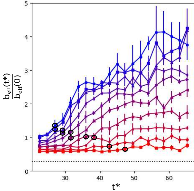
FIG. 14. Evolution of the effective filament width b_{\text{eff}} [cf. Eq. (8)] normalized to its initial value for \epsilon^* = 0 - 0.045 (blue to red). Black circles indicate the onset of nonlinearity, where Eq. (17) is first satisfied. The value of b_{\text{eff}} corresponding to a single pixel is also shown (dotted).
