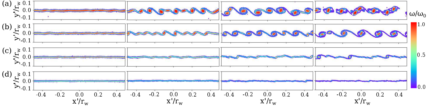
FIG. 12. Measurements of the vorticity \omega (color map) for \epsilon^* = (a) 0, (b) 0.015, (c) 0.03, and (d) 0.045 at times t^* = 22.5, 33.75, 45, \text{ and } 56.25 (left to right).
