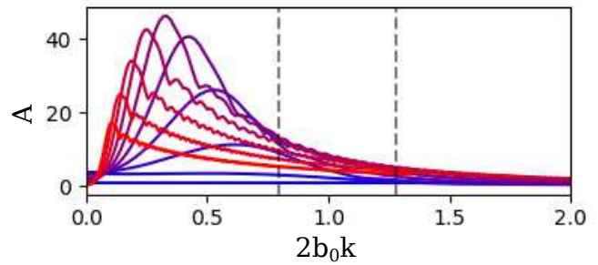
FIG. 7. Wave slope amplification spectrum A(k) over time t^* = 0 - 50 (blue to red) for \epsilon^* = 0.03 . Dashed lines indicate 2b_0k_m = 0.797 and 2b_0k_c = 1.278 .
